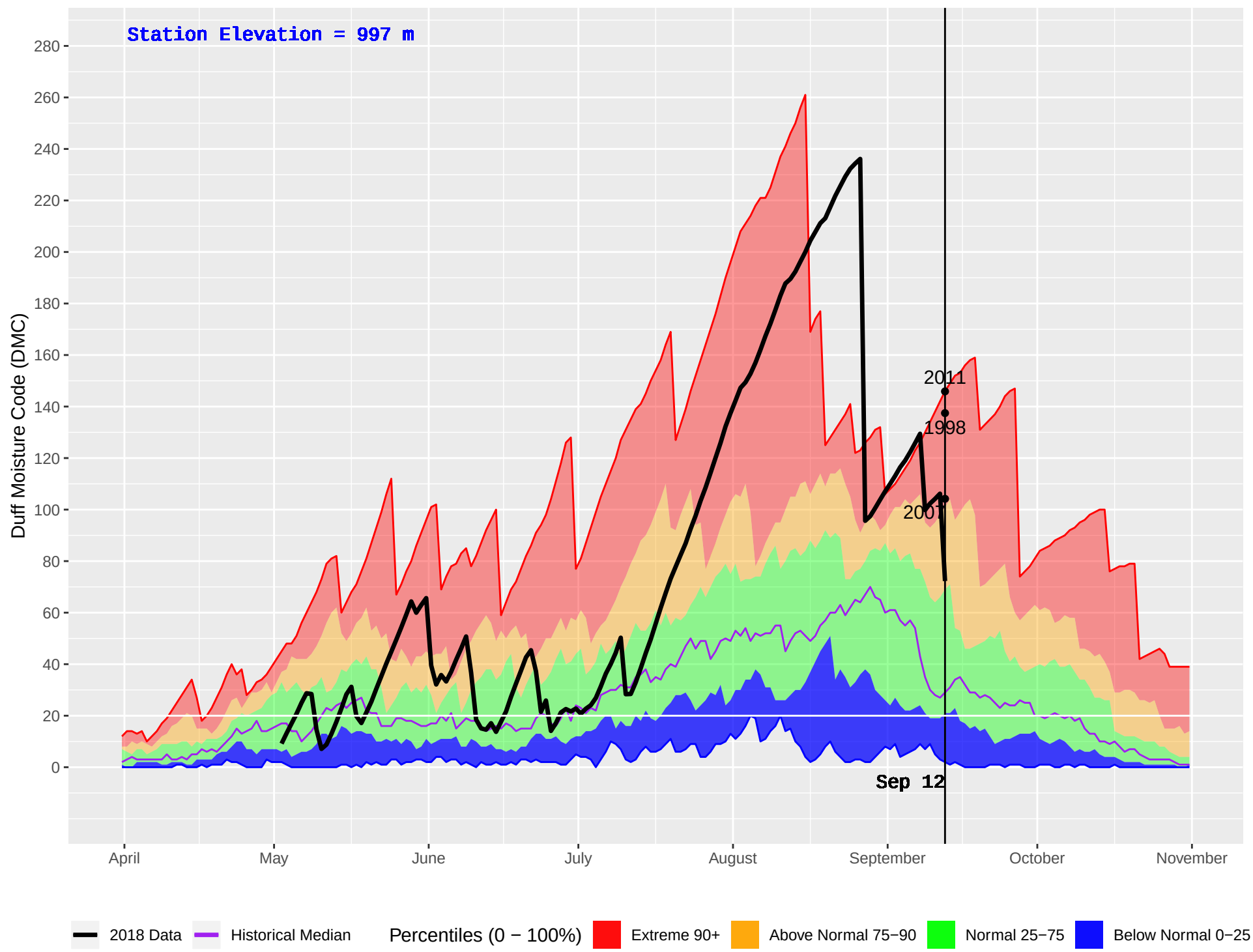
SMALLWOOD (404) : Historical (1991–2016) and Current (2018) Daily Duff Moisture Code (DMC)
