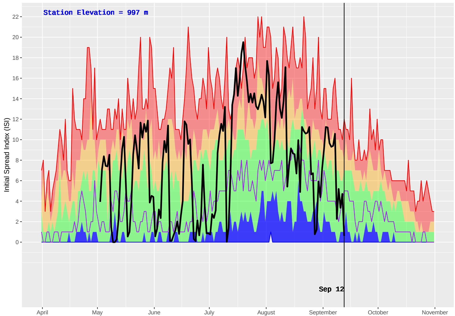
SMALLWOOD (404) : Historical (1991–2016) and Current (2018) Daily Initial Spread Index (ISI)
