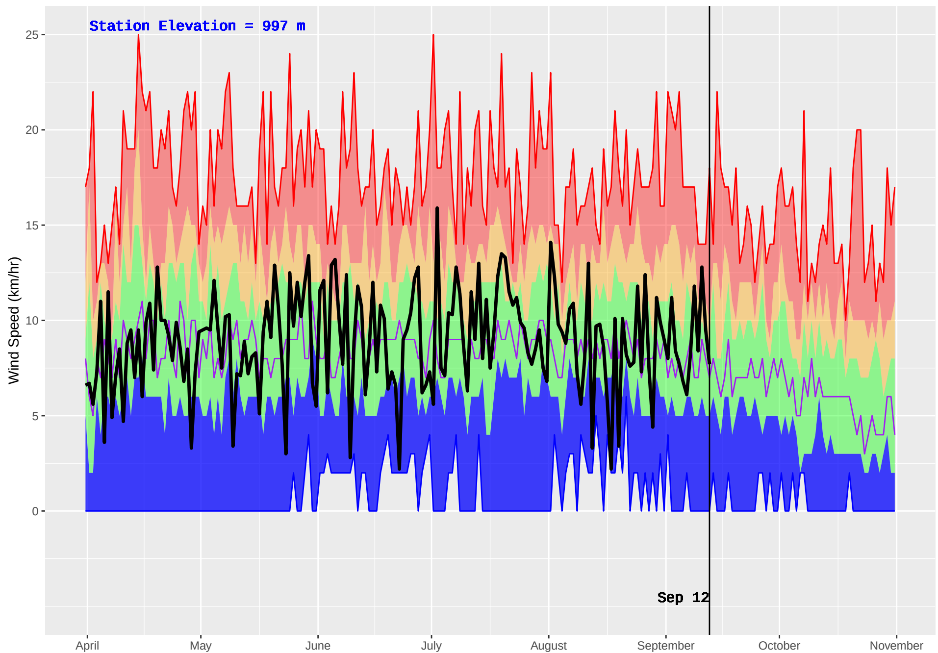
SMALLWOOD (404) : Historical (1991–2016) and Current (2018) Daily Wind Speed
